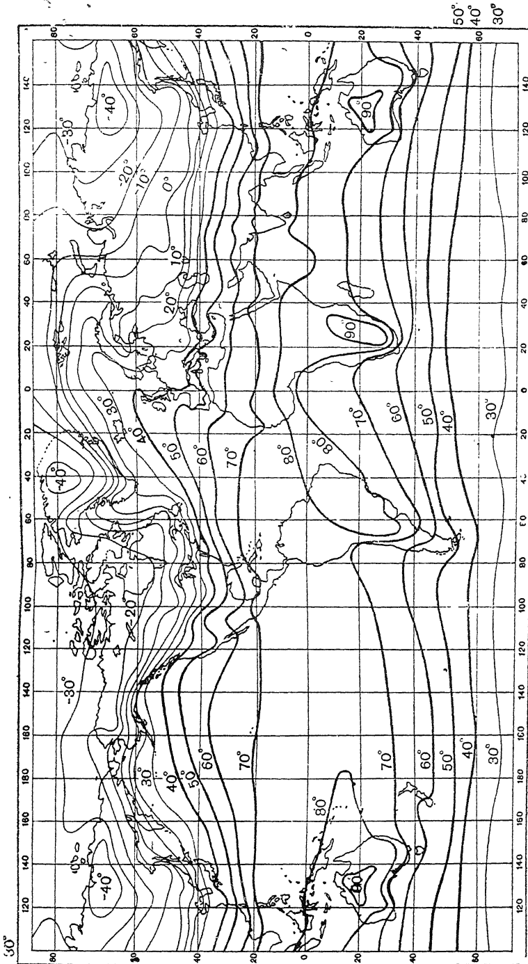
January isotherms (After Buchan, Mohn and others.)
